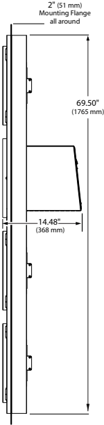
F2GBOF-7 EXTERIOR/OUTSIDE SIDE VIEW CUSTOMER SIDE
