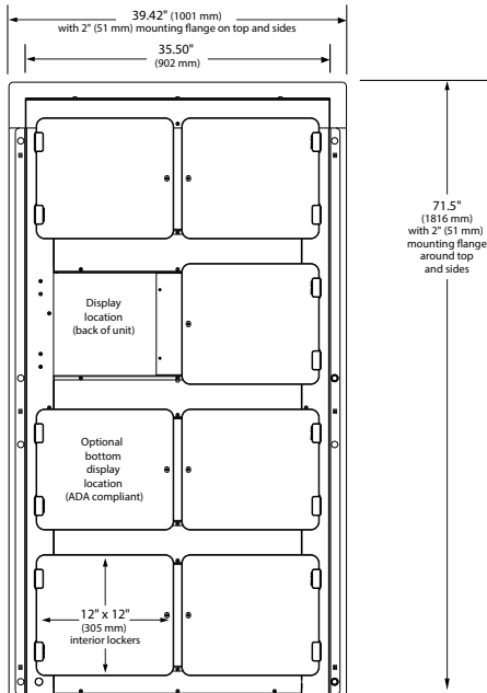
F2GBOB-7 (Standard Ambient Operation) INTERIOR/INSIDE VIEW OPERATOR SIDE
