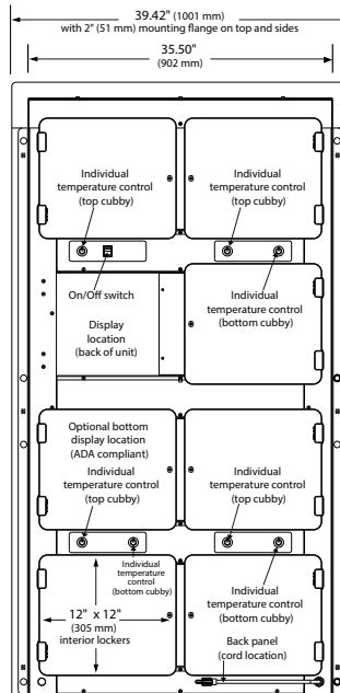
F2GBOB-7 (Optional Heated Operator) INTERIOR/INSIDE VIEW OPERATOR SIDE
