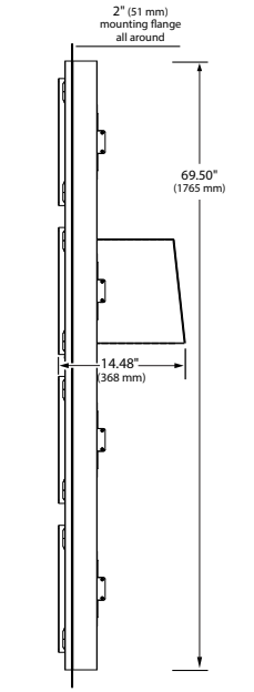
F2GBOF-11 EXTERIOR/OUTSIDE SIDE VIEW CUSTOMER SIDE
