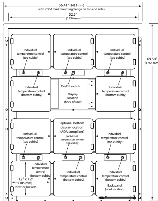
F2GBOB-11 (Optional Heated Operation) INTERIOR/INSIDE VIEW OPERATOR SIDE
