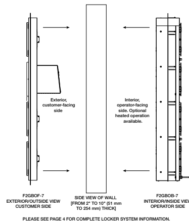
F2GBOF-7 shown from exterior customer side, mounted into a building wall.
