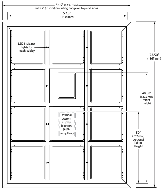
F2GBOF-11 EXTERIOR/OUTSIDE VIEW CUSTOMER SIDE
