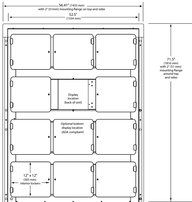
F2GBOB-11 (Standard Ambient Operation) INTERIOR/INSIDE VIEW OPERATOR SIDE
