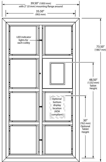
F2GBOF-7 EXTERIOR/OUTSIDE VIEW CUSTOMER SIDE
