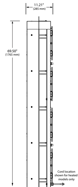
F2GBOB-7 INTERIOR/INSIDE SIDE VIEW OPERATOR SIDE
