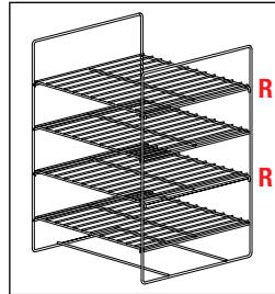
4-Shelf Multi-Purpose Rack FDW4SMP (Max. 457 x 330 mm) (Half-Size Sheet Pans fit FDWDE-2 and -2X models only) (95 mm between shelves)
