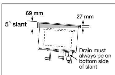
Slant Option for CWBR-S1, CWBX-S1, CWBR-S2, CWBX-S2, CWBR-S3, CWBX-S3, CWBR-S4, CWBX-S4
