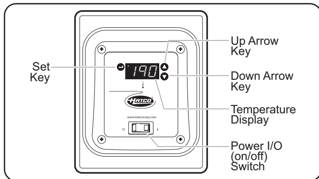
Control Box with Digital Temperature Controller
