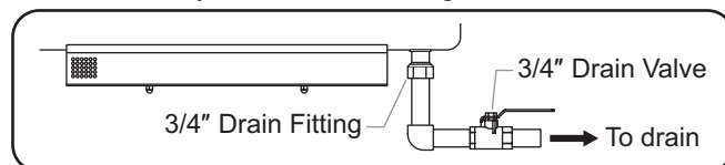
Drain Connection
