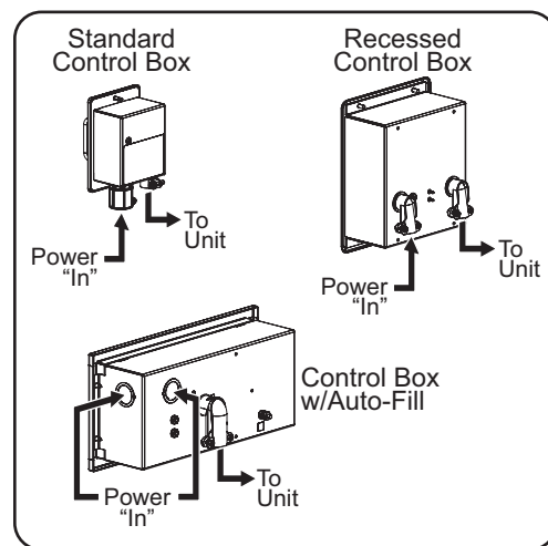
Control Box Electrical Connections
