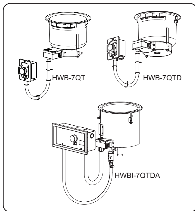
HWB-7QT, HWB-7QTD, and HWBI-7QT Models
